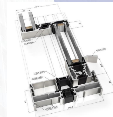
Sliding Window Thermal Break Profile
