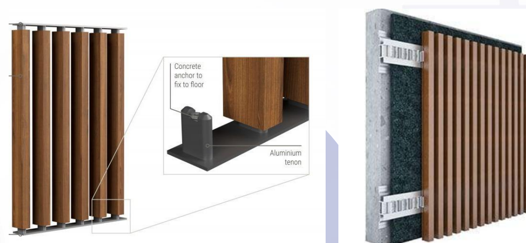
Wooden Finish Aluminium Louver
